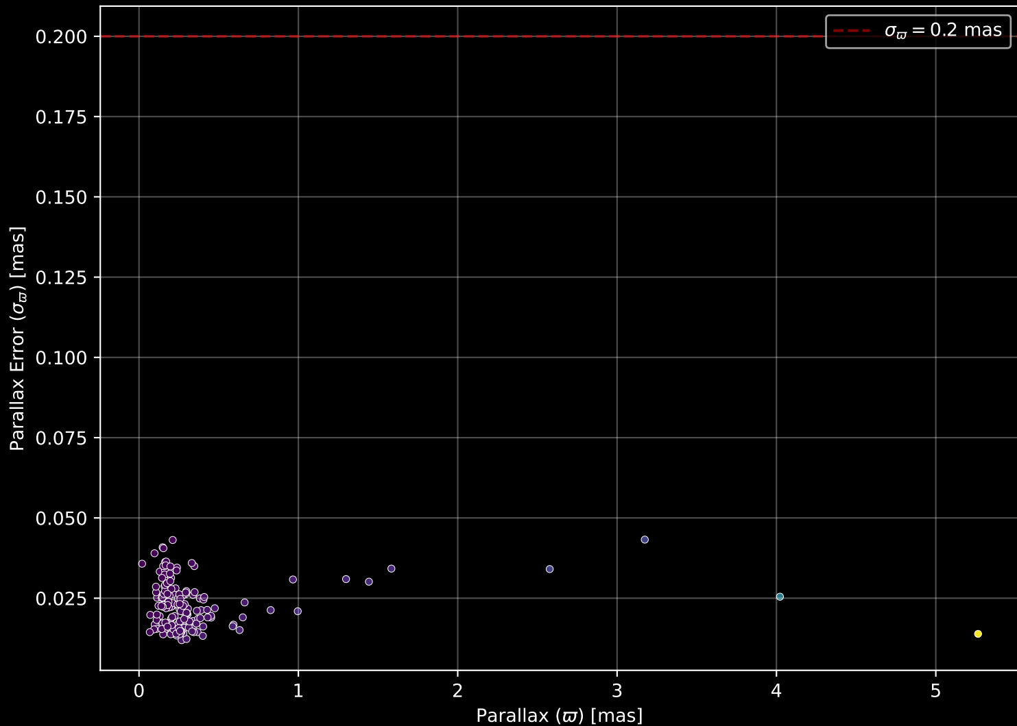
APOGEE DR17 Field: [Berkeley_18_btx] Parallax Quality (n= 168)
