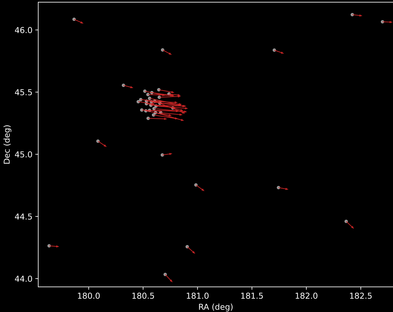
APOGEE DR17 Cluster 6 Proper Motion Vectors (n=39)
