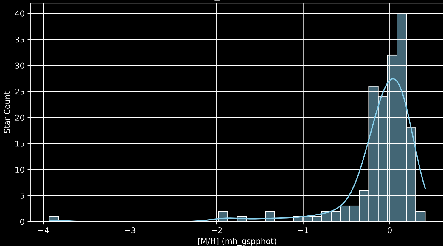
APOGEE DR17 Field: [Berkeley_18_btx [M/H] (mh_gspphot) (n= 167)
