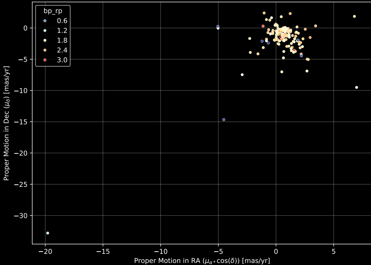
APOGEE DR17 Field: [Berkeley_18_btx] Proper Motion Diagram (n= 168)
