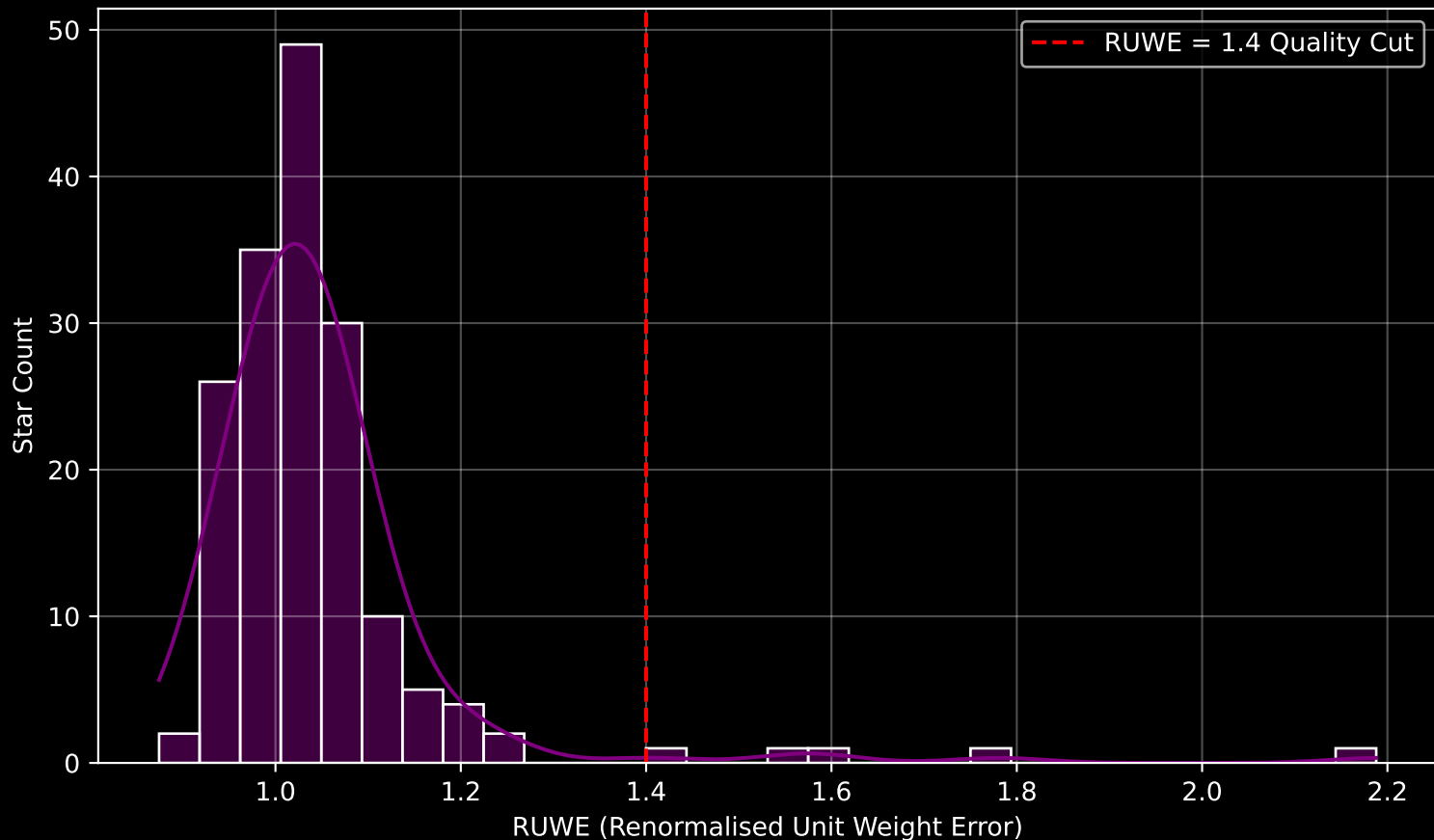
GAPOGEE DR17 Field [Berkeley_18_btx] RUWE Distribution (n= 168)
